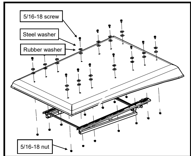
Fig. 4b (Attach Canopy to Frame)
